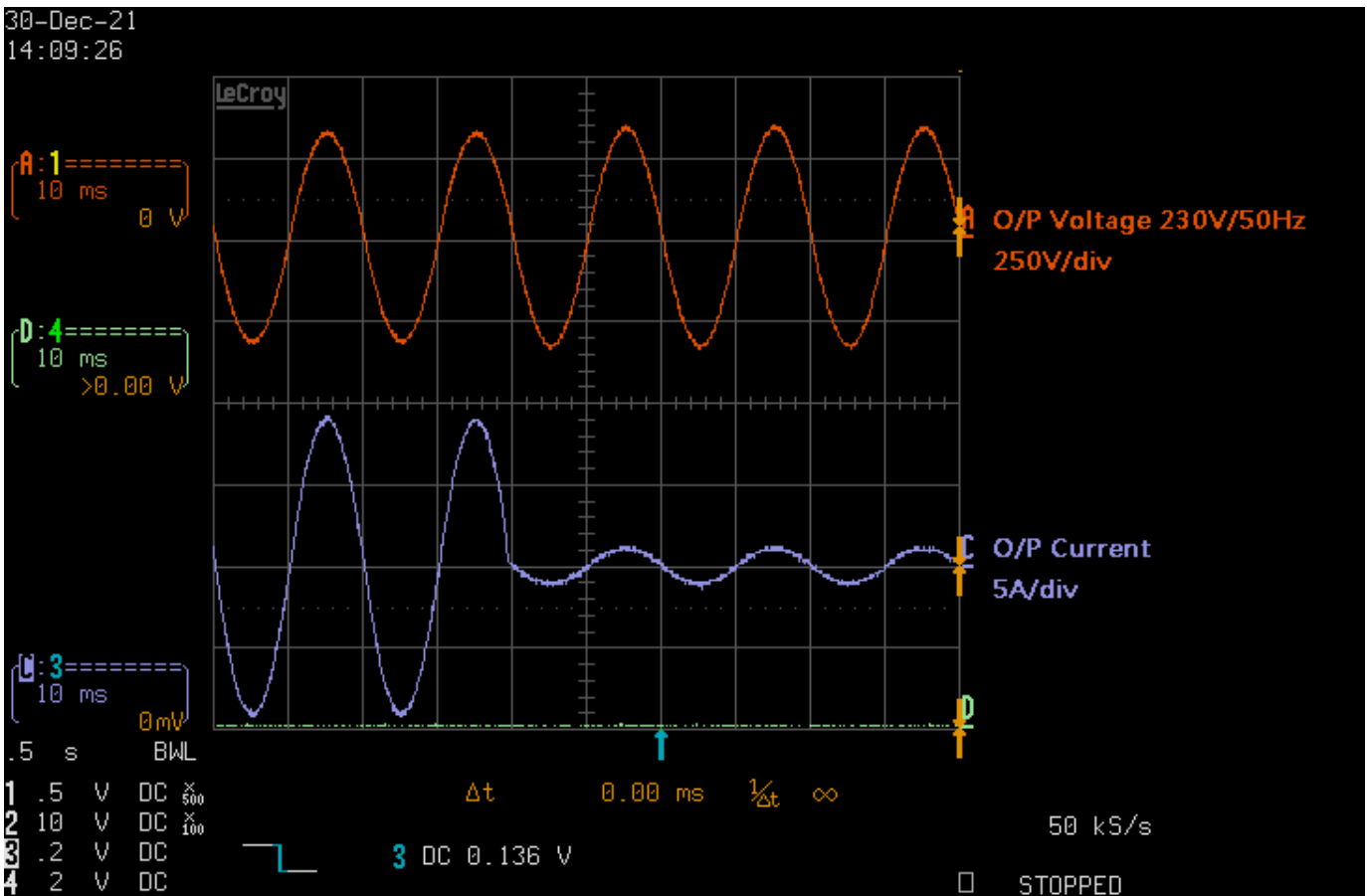
Test6: 1450W_to_150W transient response
