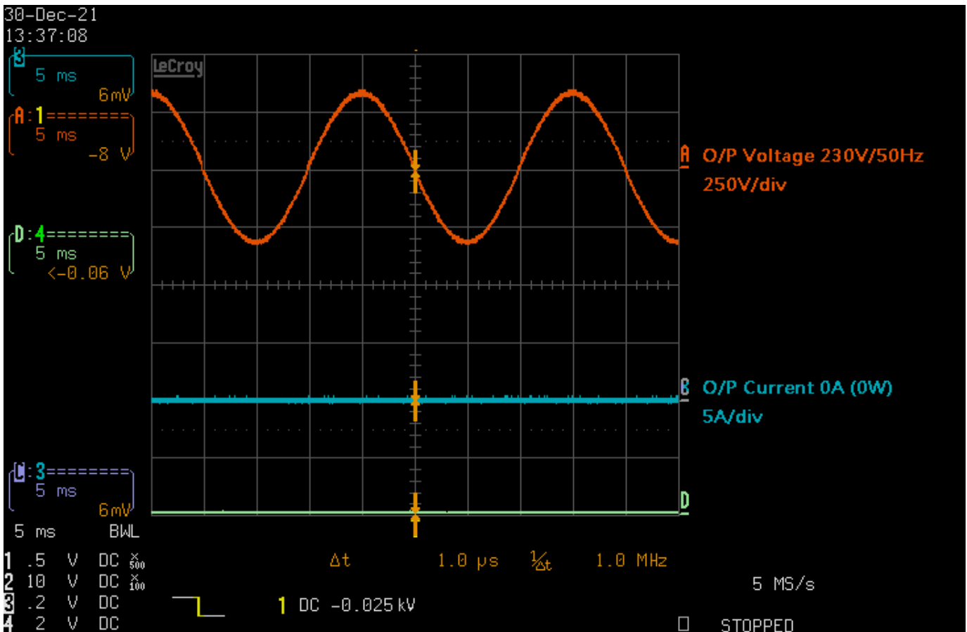
Test4: 0W level
