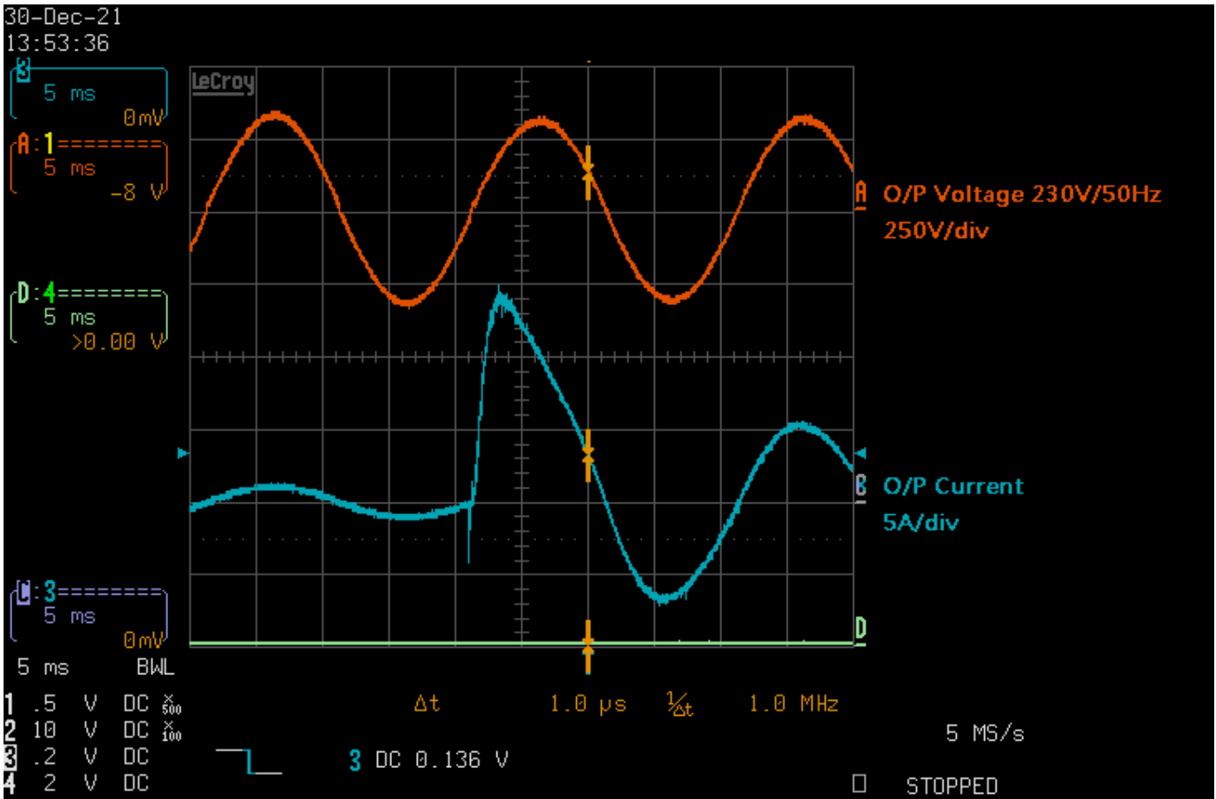
Test5: 150W_to_2000W transient response
