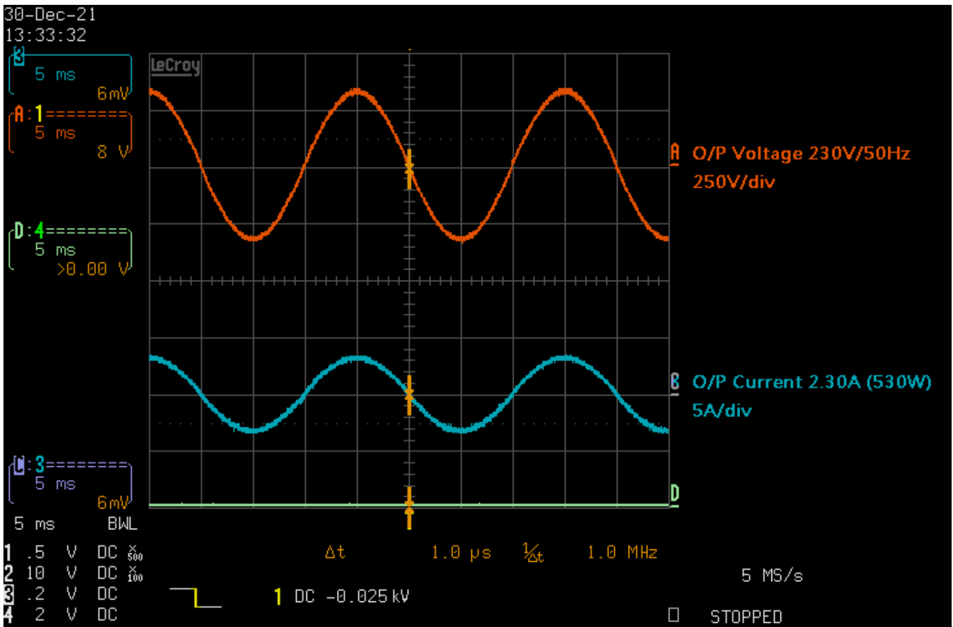
Test3: 530W level
